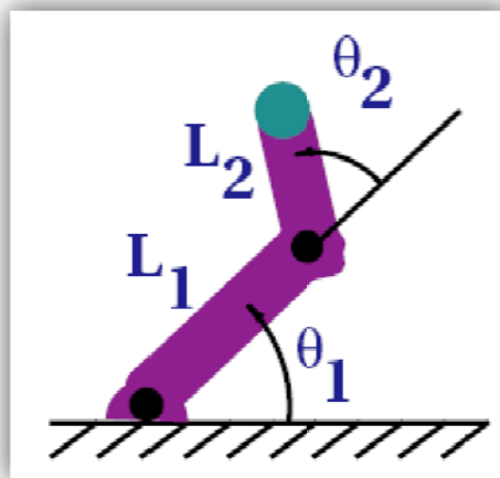
Figure 2-7: Forward kinematics
