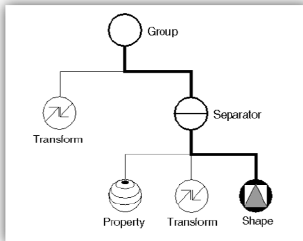
Figure 4-1: Sample scene graph. From (7).
